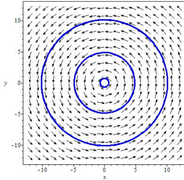
Figure 2: Three limit cycles for \varepsilon = 10^{-9}
